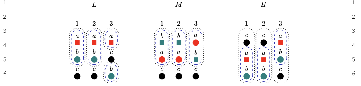
FIGURE 2.—Firms 1, 2, and 3's preference orderings over the three alternatives, at the three states, L , M , and H . For each state, the allocation chosen by SCF f^* in Ex. 3 is indicated by a square. The acceptability correspondence A from Ex. 1 is shown by the dotted lines, and is not maximally safe for this SCF. Acceptability correspondence A^* in Ex. 3 is maximally safe, and is represented by the dashed lines in the figure.
