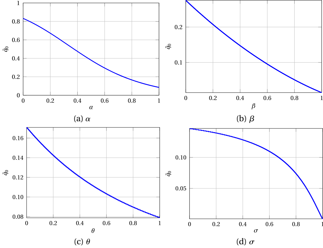
FIGURE S.1. Baseline values \psi^N = 0.5 , \alpha = 0.9 , \beta = 0.5 , \theta = 0.3 , \sigma = 0.5 , r = 0.3 , \rho = 0.5 .
