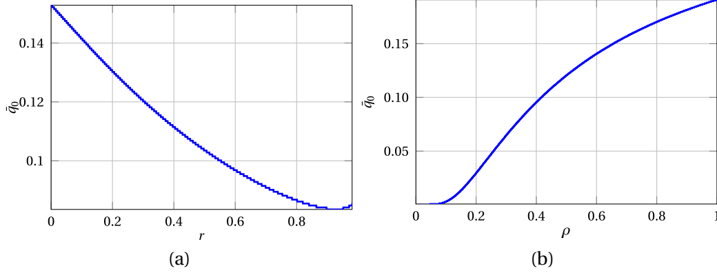
FIGURE S.2. (a) Case A_1 > 0, r ; (b) Case A_1 > 0, \rho .
