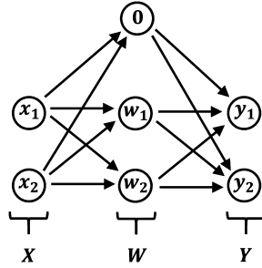
FIGURE 4. Network associated with a hedonic model.
