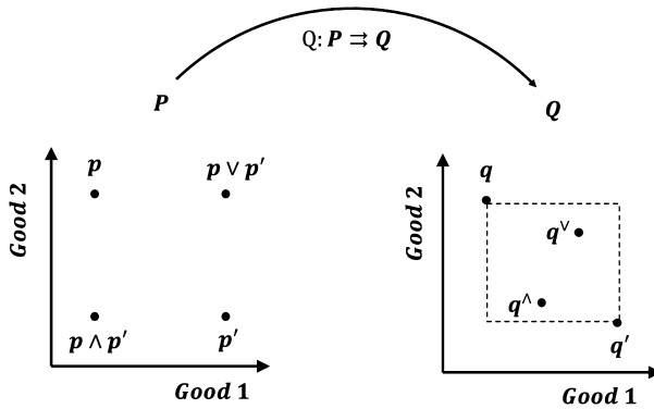
FIGURE 1. An illustration of the unified gross substitutes property with two goods. Q is a correspondence between the set of prices on the left and the set of quantities on the right with q \in Q(p) and q' \in Q(p') . Definition 1 imposes that there exists a q^\vee \in Q(p \vee p') , smaller than the top-right border of the rectangle drawn in the set of quantities, and a q^\wedge \in Q(p \wedge p') larger than the bottom-left border.
