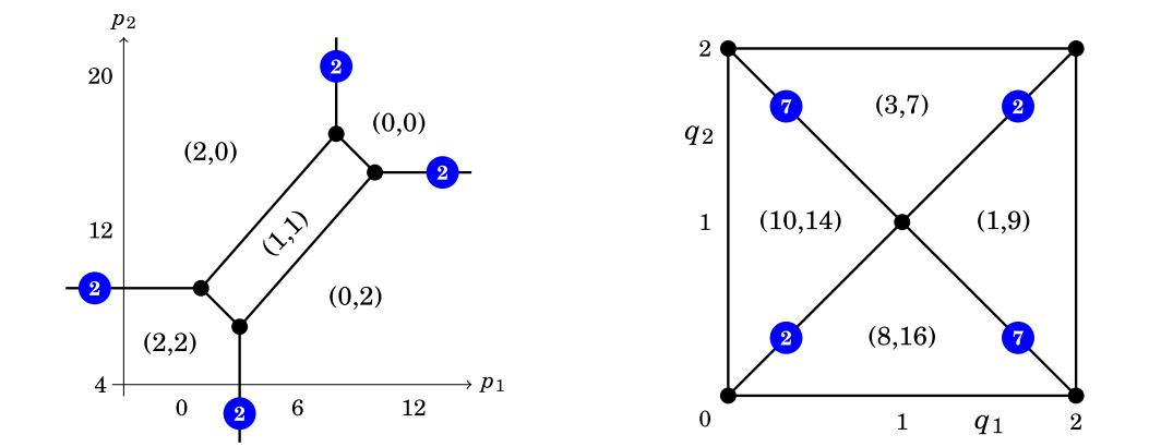
FIGURE 2. The left panel shows -\partial V and the right panel shows \partial U . Vertices in one graph correspond to regions in the dual graph and their locations produce the labels of the dual regions. In both graphs, the difference in labels between two adjacent regions is the weight (the white number in the blue disk) times the normal to the regions' common edge. Edges in one graph correspond to perpendicular edges in the dual graph, and their weights equal the dual edge's length.
