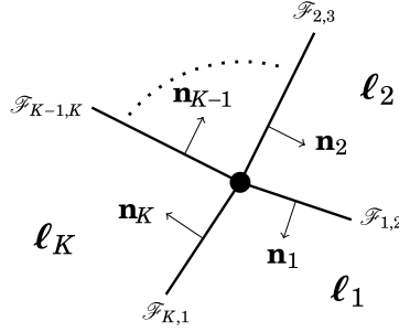
FIGURE 3. Balancedness and normal labeling.
