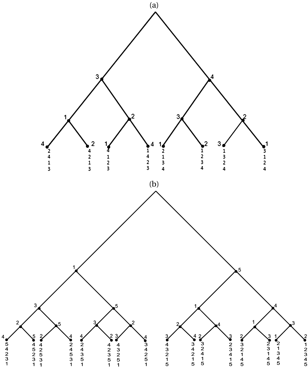
FIGURE 3. (a) A domain violating condition (16) (b) A domain violating condition (15).
