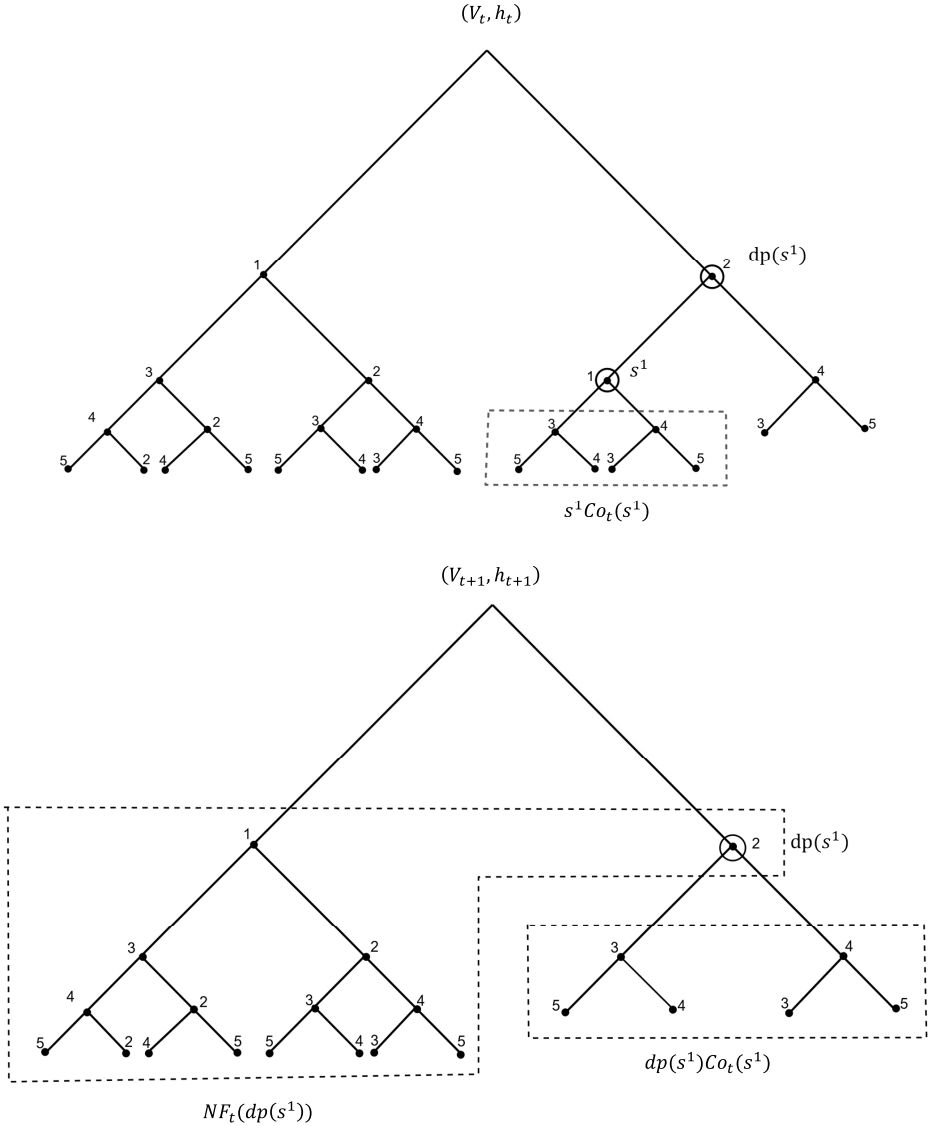
FIGURE 4. Constructing the sequence (V_t, h_t)
