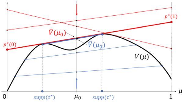
FIGURE 1. The concave closure and the concave envelope at \mu_0 in the binary-state case. The concave closure is the inner construction of the convex hull of the graph of V : It involves maximizing the value at \mu_0 over all convex combinations of points on the graph of V (exemplified by blue lines in the figure). The concave envelope is the outer construction of the convex hull of the graph of V : It involves minimizing the value at \mu_0 over all affine functions lying above the graph of V (exemplified by the red lines in the figure).
