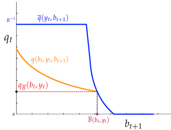
FIGURE 6. The x axis features different levels of debt issuance b_{t+1} . The y axis features the possible realizations of debt prices after history h^t given y_t for each value of b_{t+1} ; \bar{q}(y_t, b_{t+1}) is the best equilibrium price function; \bar{B}(b_t, y_t) is the maximum debt issuance such that the government is indifferent between defaulting and repaying; q_{\bar{B}}(b_t, y_t) is the lowest (certain) equilibrium consistent price realization with no default.
