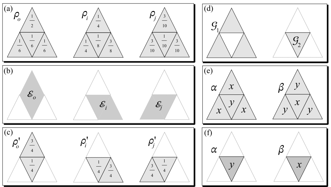
FIGURE 1. An example of complementary ignorance: (a) the prior beliefs of the three agents, (b) the events they observe, (c) their posterior beliefs, (d) the partition \mathfrak{G} = \{\mathcal{G}_1, \mathcal{G}_2\} , (e) the acts \alpha and \beta , ex ante , and (f) the acts \alpha and \beta in light of the combined information of all agents.
