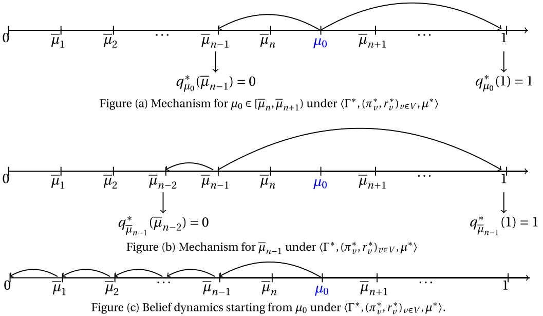
FIGURE 1. Mechanism and belief dynamics under \langle \Gamma^*, (\pi_v^*, r_v^*)_{v \in V}, \mu^* \rangle as a function of \mu_0 .
