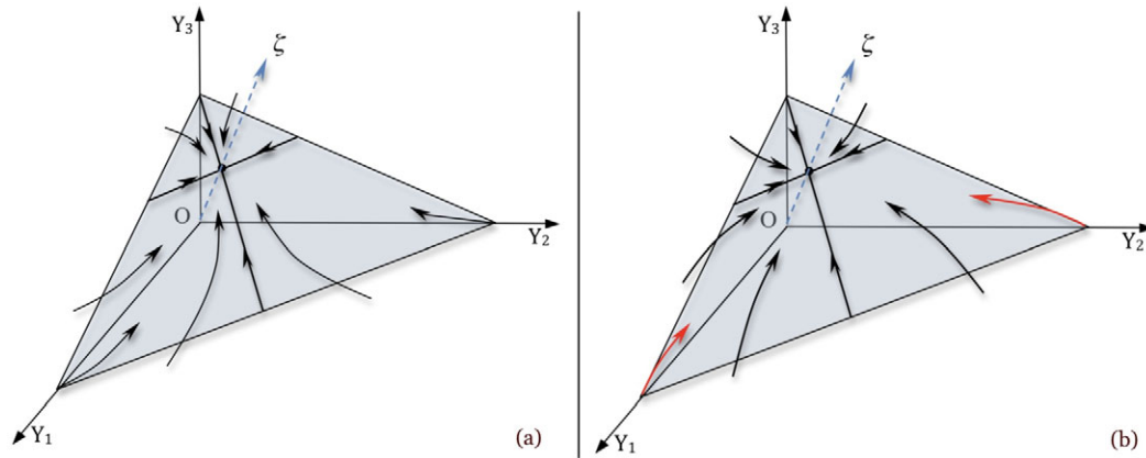
FIGURE 3. Vector field of the velocity of the detrended trajectories when b > 0 (part (a)) and b = 0 (part (b)) in the example of Section 2.2.
