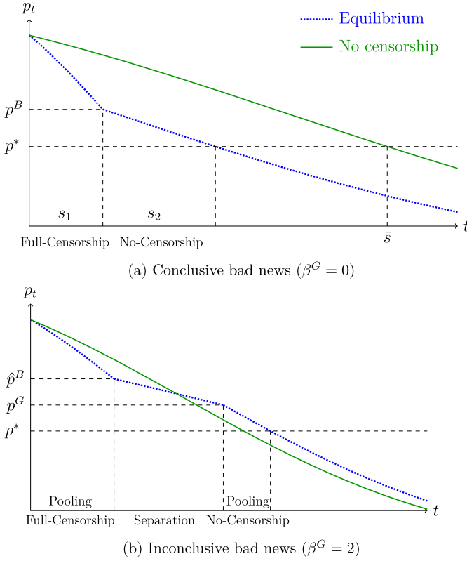
FIGURE 1. The belief drifting process (\gamma, \beta^B, p_0, p^*, w, c, \rho) = (5, 3.5, 0.75, 0.4, 10, 1, 6) .
