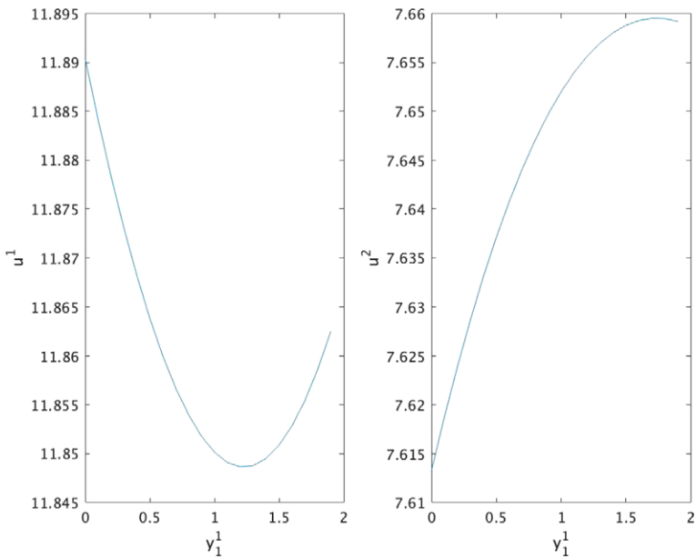
FIGURE 1. Pareto ranked ex ante utilities.
