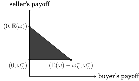
FIGURE 3. Payoffs at all sequential Bayes' correlated equilibria.
