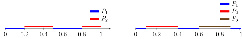
FIGURE 2. The partition of the state space \Omega = [0, 1] on the left is not laminar while the partition on the right is laminar, as the convex hull of all pairs of sets P_1 , P_2 , and P_3 are either nested or have an empty intersection.
