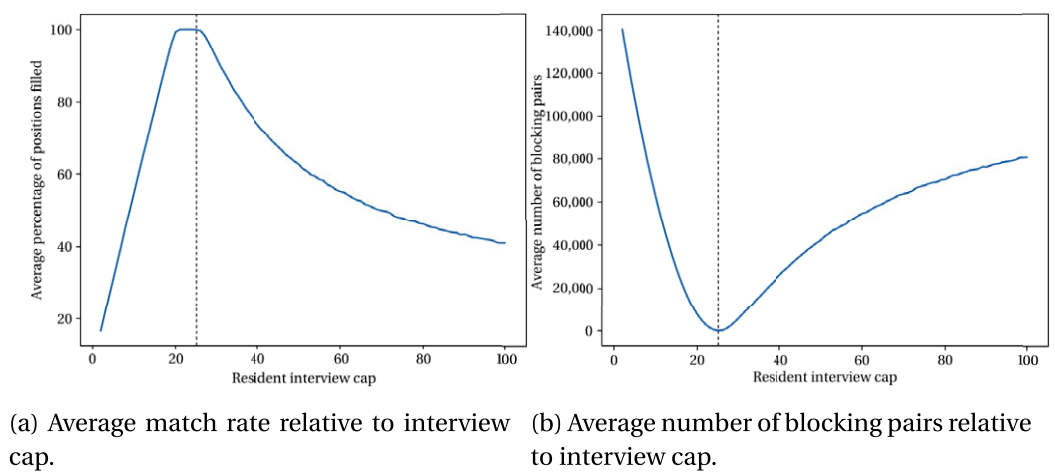
FIGURE 1. Average match rate and average number of blocking pairs relative to doctors' interview cap. In this figure, k varies from 2 to 100 with l fixed at 25 (indicated by a vertical line). When k = l , the average match rate is 99.9525% and the average number of blocking pairs is 136.08.
