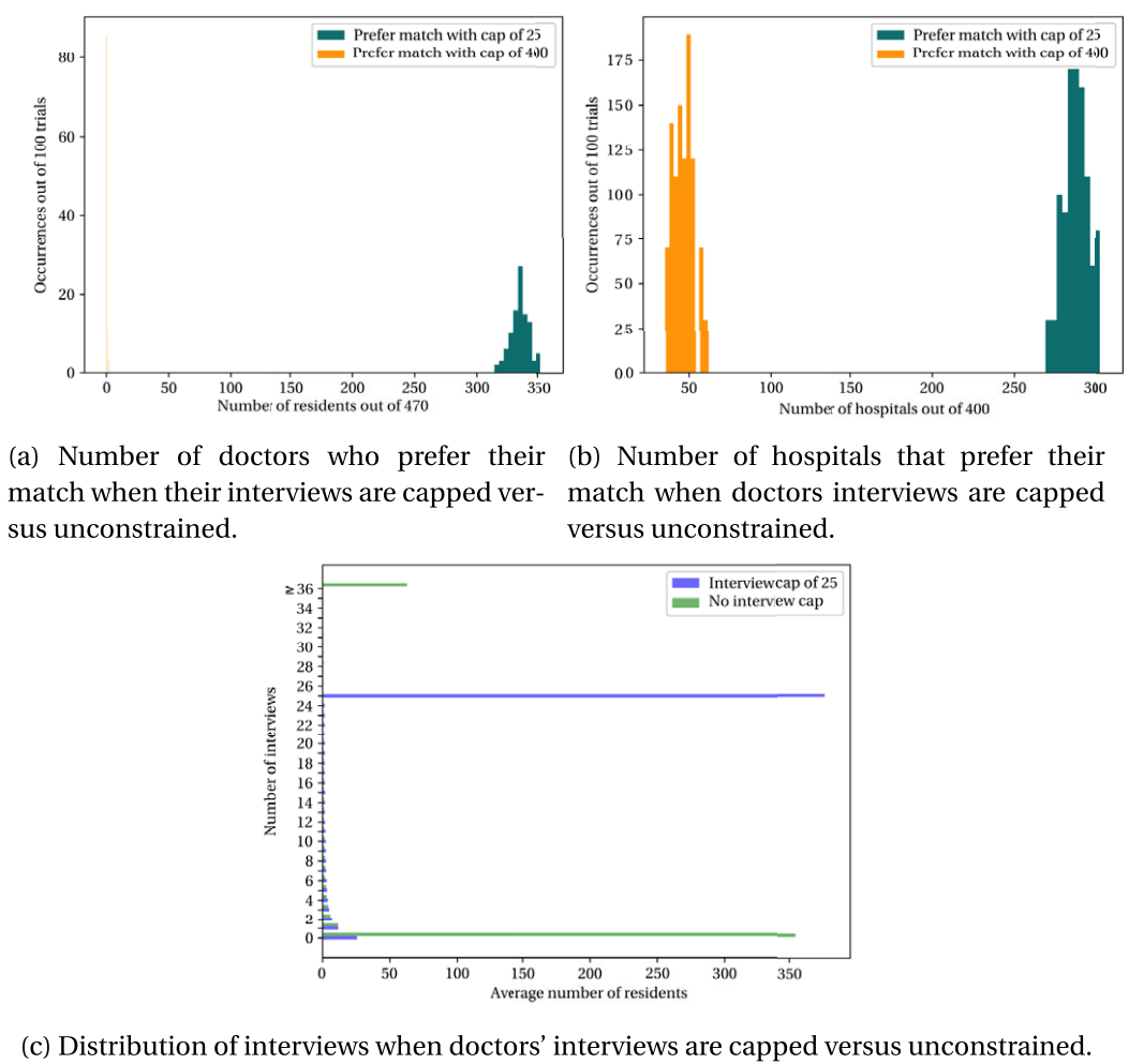
FIGURE 2. Comparison of capped versus unconstrained doctor interviews. This figure shows comparisons of the effects of the intervention of capping doctors' interview capacities at k = l versus leaving the capacities unconstrained. In (c), since the tail of the distribution without caps is very thin, the total number of doctors with 36 or more interviews is consolidated into a single bar.
