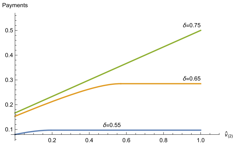
FIGURE 4. Illustration of the equilibrium payment H_{\frac{L(\Pi^*, \delta)}{n-1}} as a function of the second-highest reported valuation, for the discount factors \delta = 0.55, 0.65 , and 0.75 . Assume that there are two buyers and F is uniform on [0, 1] .
