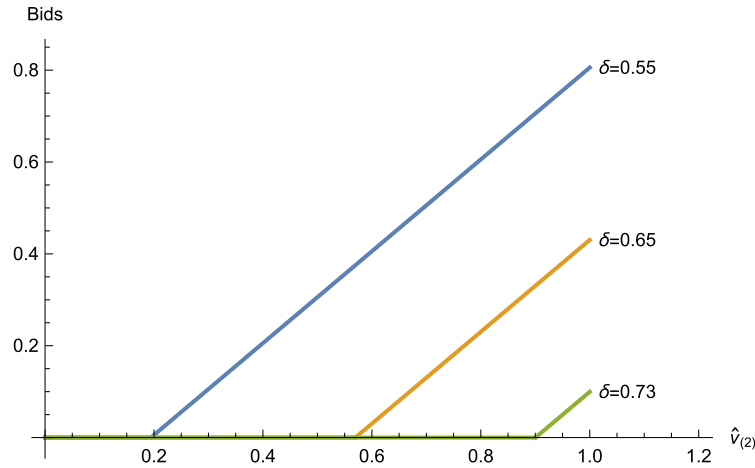
FIGURE 3. Illustration of the equilibrium bids \beta_i^* as a function of the second-highest reported valuation, for the discount factors \delta = 0.55, 0.65 , and 0.73 . Assume that there are two buyers and F is uniform on [0, 1] .
