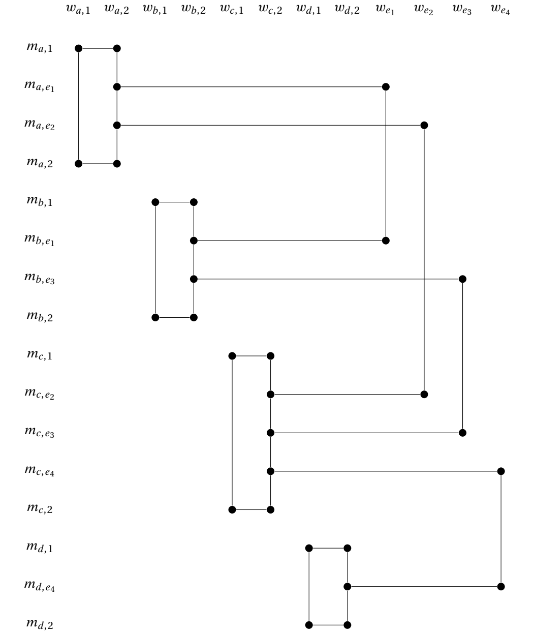
FIGURE 7. MTR-NTU instance of the graph in Figure 6.
