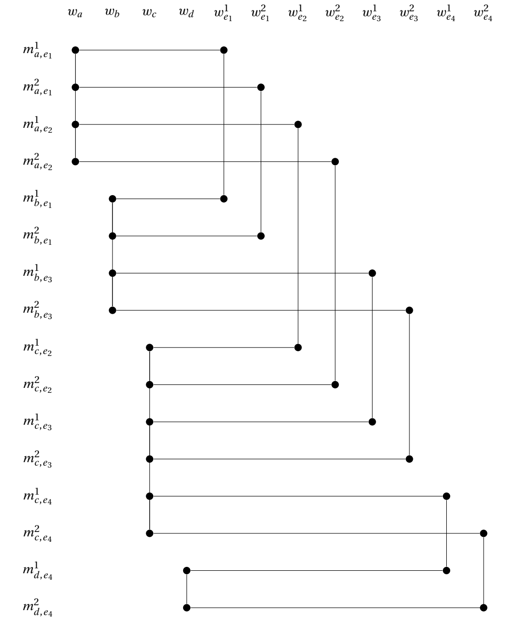
FIGURE 9. MTR-TU instance of the graph in Figure 6.
