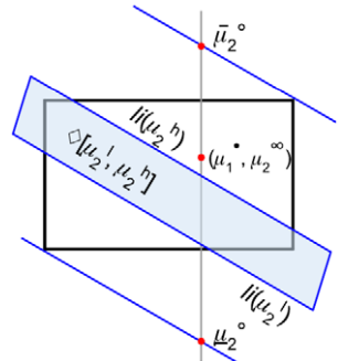
FIGURE 3. Notation for the proof of Proposition 7.
