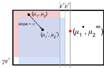
FIGURE 1. Directional derivative for data log likelihood along the vector (1, -\gamma) in the space of fundamentals implies the upper shaded region receives zero posterior probability asymptotically.
