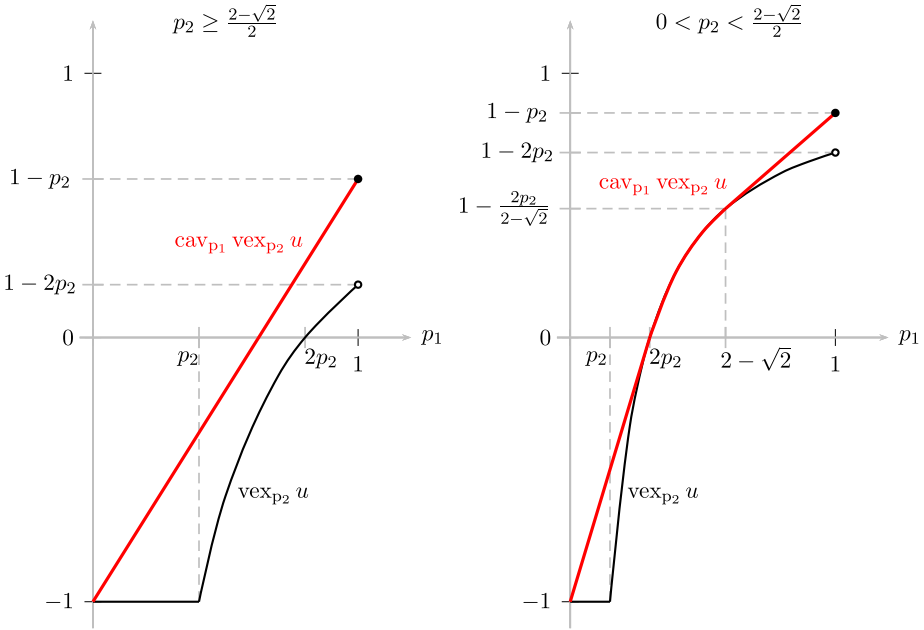
FIGURE 3. Concavification of \text{vex}_{p_2} u(p_1, p_2) .
