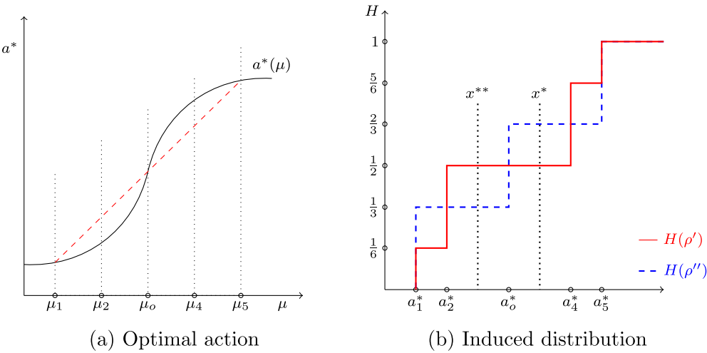
FIGURE 1. Nonconvexity/concavity and nonresponsiveness.
