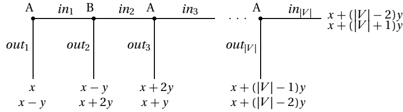
FIGURE 5. Centipede game.
