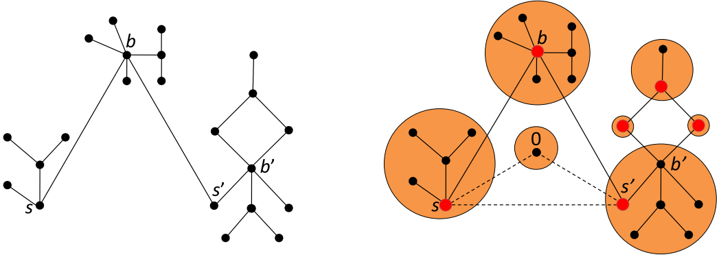
FIGURE 3. Equivalence classes for G(\{s, s'\}) and corresponding dealers.
