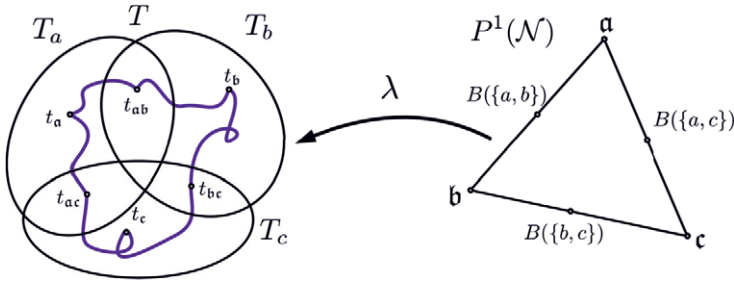
FIGURE 3. Map \lambda : P^1(\mathcal{N}) \rightarrow T carried by \mathcal{C}^{-1} , where \mathcal{C} : A \rightarrow A_0 is a carrier for covers T = \bigcup_{a \in A} T_a^f and P(\mathcal{N}) = \bigcup_{a \in A_0} \text{bst } a .
