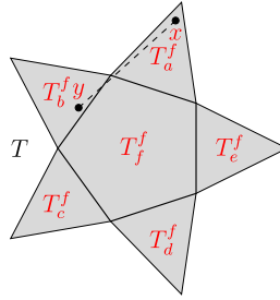
FIGURE 2. An example of a star-shaped domain T and outcome sets corresponding to f : T \rightarrow \{a, b, c, d, e, f\} that satisfy the conditions of Corollary 1 .
