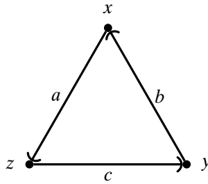
FIGURE 1. An example of a function that is monotone, but not cyclically monotone.
