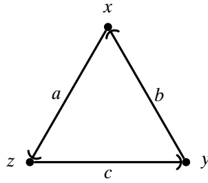
FIGURE 1. An example of a function that is monotone, but not cyclically monotone.
