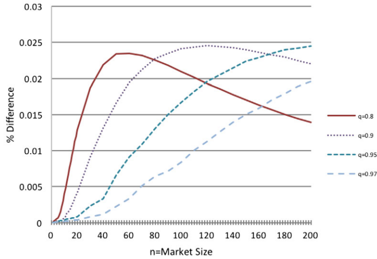
FIGURE 2. The percentage difference in expected marriages between \mu^{\text{DA}} (simulation) and \mu^{\text{SD}} (Equation (2)).
