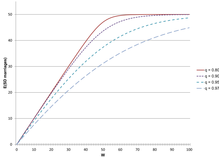
FIGURE 1. The expected number of marriages under serial dictatorship for various q(p) , fixing M = 50 .
