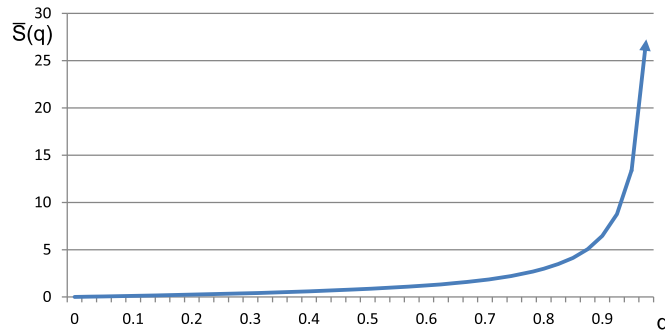
FIGURE 3. The expected number of unmatched men (women) under \mu^{\text{SD}} in large, balanced markets at prices p is \bar{S}(q(p)) .
