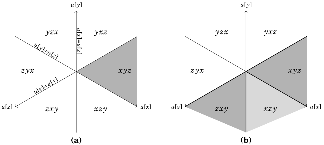
FIGURE 1. The sets of cardinal utility vectors associated with each ordering \succeq (denoted by U(\succeq) ) for X = \{x, y, z\} . (a) The set U(xyz) is shaded. (b) For the nonconvex type t = \{xyz, zxy\} , U(t) = U(xyz) \cup U(zxy) is shaded in dark and \overline{U(\text{Cons}(t))} is the union of all three shaded areas.
