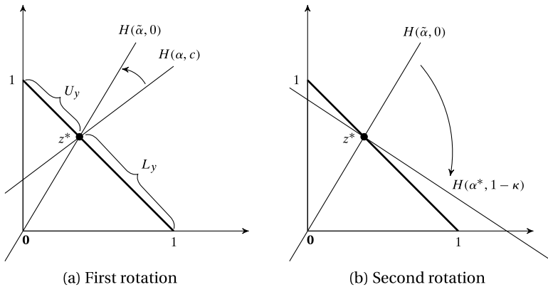
FIGURE 5. Separating hyperplanes. In panel (a), hyperplane H(\tilde{\alpha}, 0) is a rotation of H(\alpha, c) around the point z^* , which still separates L_y from U_y , but now passes through the origin. In panel (b), hyperplane H(\alpha^*, 1 - \kappa) is a rotation of H(\tilde{\alpha}, 0) around the point z^* , which intercepts the vertical axes at (1 - \kappa)\tilde{\phi}/(\tilde{\alpha}(2) + (1 - \kappa)\tilde{\phi}) and the horizontal axes at (1 - \kappa)\tilde{\phi}/(\tilde{\alpha}(1) + (1 - \kappa)\tilde{\phi}) . This hyperplane still separates L_y from U_y , but each component of the norm is between 0 and 1, and the constant is 1 - \kappa .
