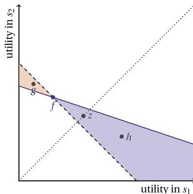
FIGURE 1. Indifference curves for \succsim and \succsim_f .
