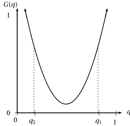
FIGURE 6. Uniqueness.
