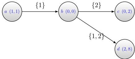
FIGURE 4. LCS differs from (C)ECB.
