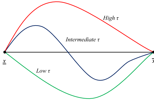
FIGURE 1. NUC. The figure depicts the behavior of the function z(\cdot, \tau, a) for three different levels of \tau : depending on \tau it can be always negative, always positive, or first positive and then negative. In all cases, it starts and ends at 0.
