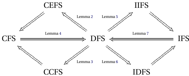
FIGURE 1. Proof strategy for Theorem A.1. (The unlabeled implications are immediate.)
