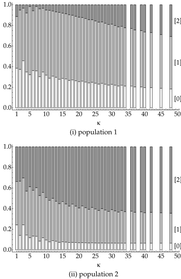
FIGURE 3. The stable interior rest point of the \text{BEP}(\tau^{\text{all}}, \kappa, \beta^{\min}) dynamic in the centipede game of length d = 4 , \kappa = 1, \dots, 50 . Stacked bars, from the bottom to the top, represent weights on strategies [0], [1], and [2].
