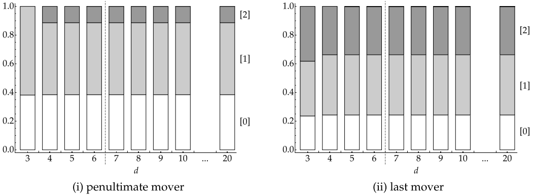
FIGURE 2. The stable rest point \xi^* = \xi^*(d) of centipede under the \text{BEP}(\tau^{\text{all}}, 1, \beta^{\min}) dynamic for game lengths d = 3, \dots, 10 and d = 20 . Stacked bars, from the bottom to the top, represent weights on strategy [0] (continue at all decision nodes), [1] (stop at the last node), [2] (stop at the second-to-last node), etc. The dashed line separates exact ( d \leq 6 ) and numerical ( d \geq 7 ) results.
