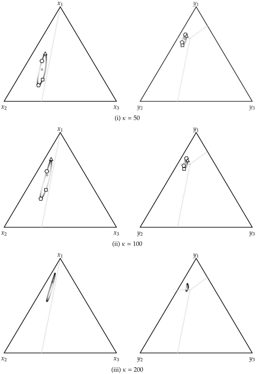
FIGURE 5. Stable cycles in centipede of length d = 4 under \text{BEP}(\tau^{\text{all}}, \kappa, \beta^{\min}) dynamics for \kappa = 50, 100 , and 200 . Lighter shading represents faster motion. The small circles represent the unstable interior rest points. For \kappa = 50 and 100 , shapes synchronize positions along the cycle.
