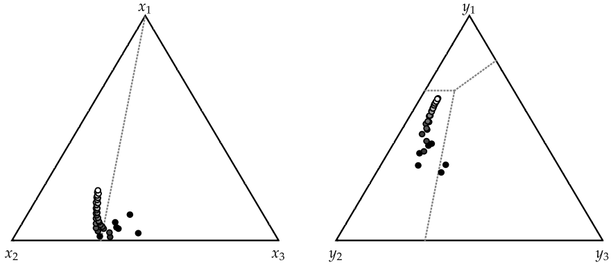
FIGURE 4. The stable interior rest point in centipede of length d = 4 under \text{BEP}(\tau^{\text{all}}, \kappa, \beta^{\min}) dynamics for \kappa = 1, \dots, 34 trials of each tested strategy. Lighter shading corresponds to larger numbers of trials. Dashed lines represent boundaries of best response regions.
