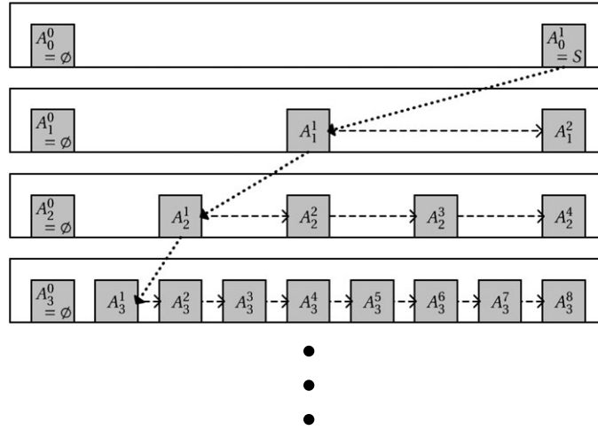
FIGURE 3. Proof of Theorem 2 . More specifically, this is the structure of Step 1 and Step 2 of the Supercabinet Construction Lemma ( Lemma 18 ). We construct events A_q^p , where q \in \{0, 1, \dots\} and p \in \{0, 1, \dots, 2^q\} , such that we intend to associate each A_q^p with the measure p/2^q . For the dotted lines, we use our halving technique from Appendix F . For the dashed lines, we use our disjoint-pair technique from Appendix E . The rest of the proof is dedicated to establishing that the associated likelihood equivalence classes are in fact a supercabinet; this is where we require 3-AS.
