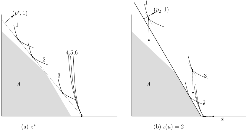
FIGURE 1. Rule \Phi .
