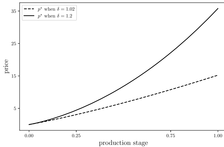
FIGURE 3. Equilibrium price functions when c(\ell) = e^{\theta\ell} - 1 .
