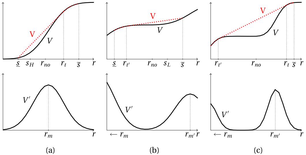
FIGURE 2. Sender's utility V and concave closure \bar{V} when derivative V' is (a) unimodal and (b), (c) bimodal.
