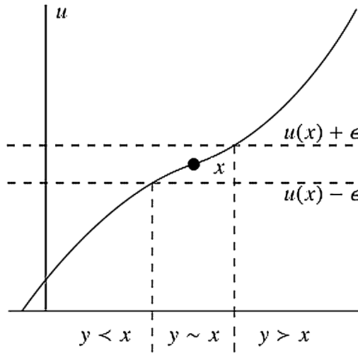
FIGURE 4. A semioorder representation.
