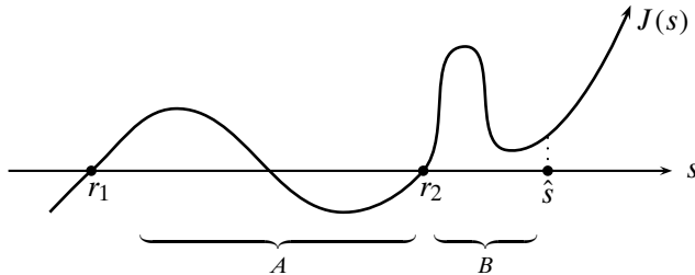
FIGURE 4. Gains and losses from reserve prices r_1 < r_2 .
