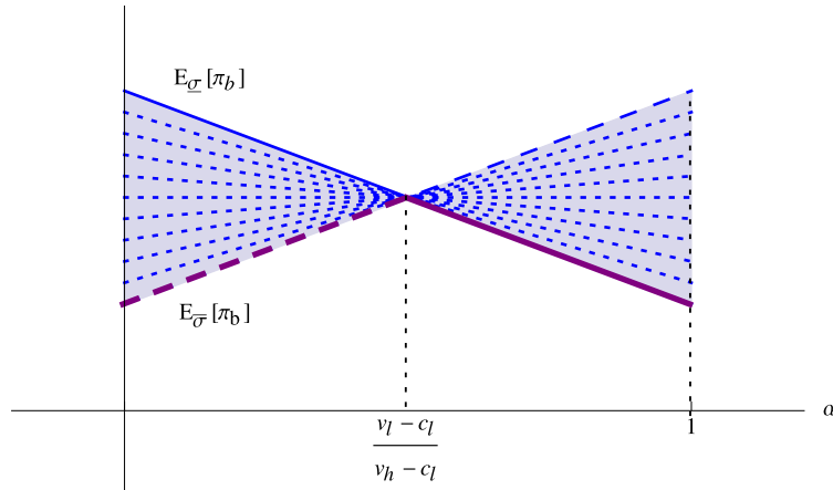
FIGURE 1. Expected payoffs E_\sigma[\pi_b] for \sigma \in [\underline{\sigma}, \overline{\sigma}] .
