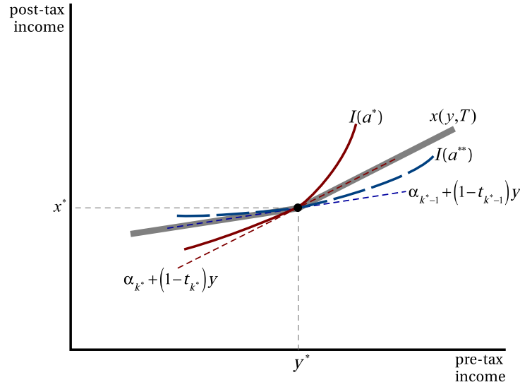
FIGURE 3. Figure for Lemma 4.
