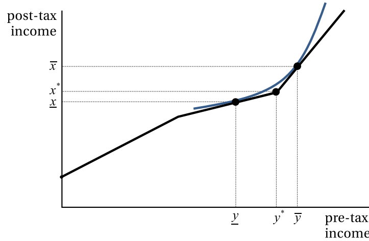
FIGURE 1. Figure for Theorem 1.
