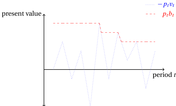
FIGURE 1. Envelope.
