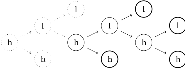
FIGURE 2. Contingent truncation.
