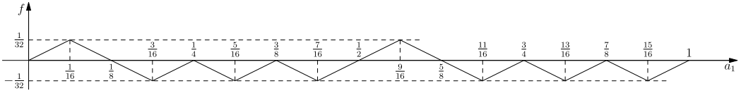
FIGURE 4. The graph of f((a_1, 0), b) .
