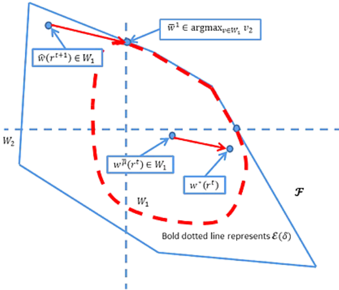
FIGURE 4. The vector from w^{\tilde{\mu}}(r^t) to w^*(r^t) is parallel to the one from \hat{w}(r^{t+1}) to \bar{w}^1 .
