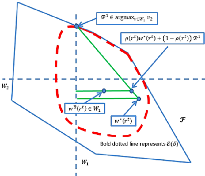
FIGURE 5. \rho(r^t)w^*(r^t) + (1 - \rho(r^t))\bar{w}^1 and w^{\tilde{\mu}}(r^t) have the same value for player 2.
