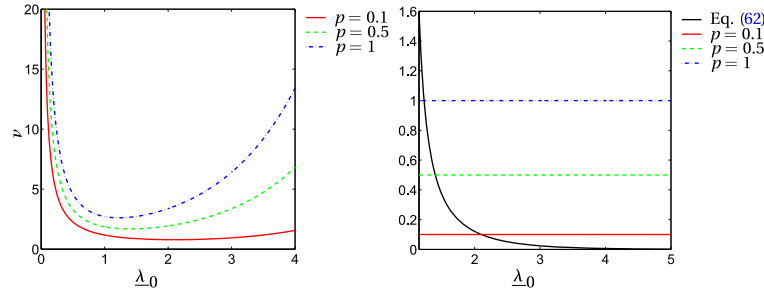
FIGURE 11. Left panel: The traveling wave velocity \nu as a function of \lambda_0 for different values of p = 0.1 , p = 0.5 , and p = 1 . Right panel: The \nu minimizing value of \lambda_0 for the same values of p . The figures show that the minimizing value of \lambda_0 is decreasing for increasing values of p and, consequently, the front of the traveling wave becomes steeper. Moreover, the velocity \nu of the traveling wave increases with increasing values of p .
