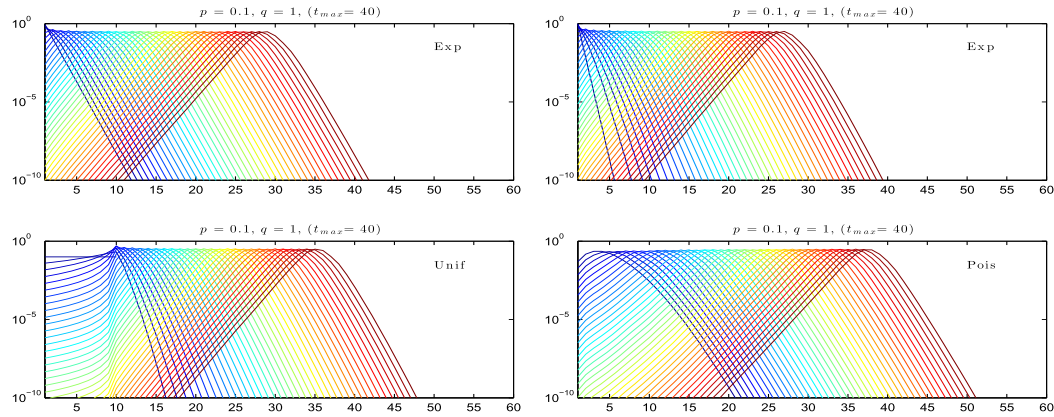
FIGURE 4. Examples of numerical solutions of the system of ODEs in (14) with different initial conditions. In all cases, we set p = 0.1 , q = 1 , and \log \bar{A} = 1 , yielding \lambda = 2.1 (cf. (20)). The top left panel shows the traveling wave with an exponential decay with \lambda = 2.1 . The other three panels show the transition from different initial conditions. The top right panel shows an initial distribution decaying exponentially with an exponent \lambda = 5 . The tail of the distribution increases until it reaches the stationary value of \lambda = 2.1 , as in the top left panel. The bottom left panel shows the transition from a uniform initial distribution on the interval [0, 1] . The bottom right panel shows the transition from a Poisson initial distribution with parameter 3. In all cases, the distribution converges to the traveling wave in the top left panel.
