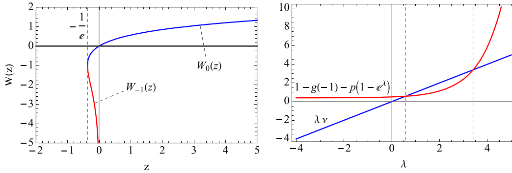
FIGURE 9. Left panel: The two real Lambert W functions. Right panel: The two real roots \bar{\lambda}_0 and \bar{\lambda}_{-1} solving (46) for \nu = 1 , g(-1) = 0.5 , and p = 0.1 indicated with dashed lines, and given by \bar{\lambda}_0 = 0.5783 and \bar{\lambda}_{-1} = 3.4018 .
