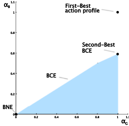
FIGURE 1. BNE and set of BCE with low accuracy: q = \frac{1}{5} .
