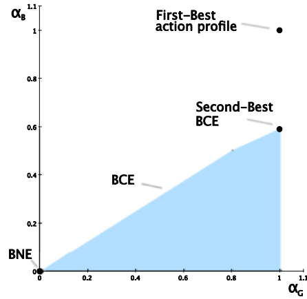
FIGURE 1. BNE and set of BCE with low accuracy: q = \frac{1}{5} .
