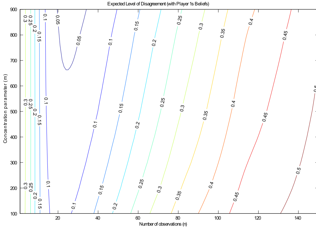
FIGURE 3. Ex ante expected disagreement in the binary example of Section 3.2 for \epsilon = \lambda = 1/m .
