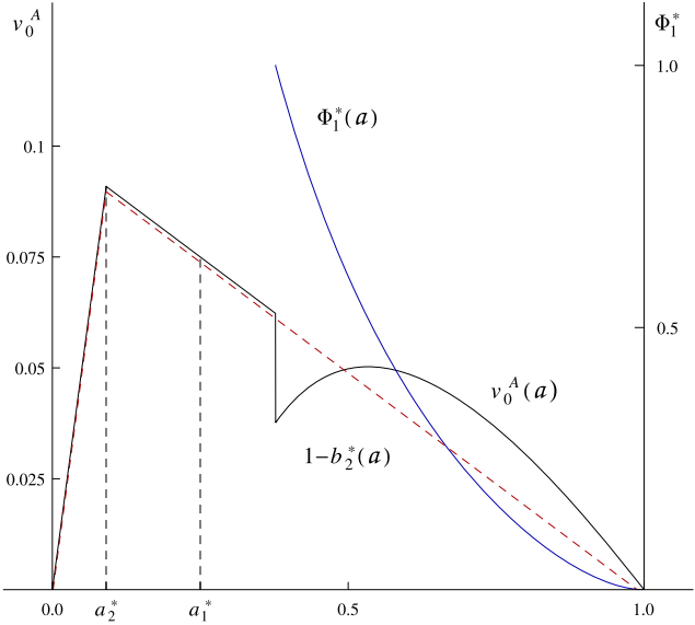
FIGURE 7. (\beta_1, r_1^B, r_2^B) = (0.3, 0.333, 0.1) .
