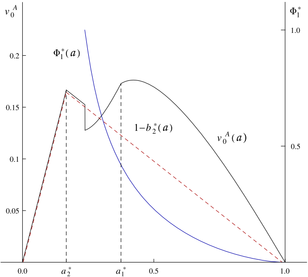
FIGURE 8. (\beta_1, r_1^B, r_2^B) = (0.575, 0.6, 0.2) .
